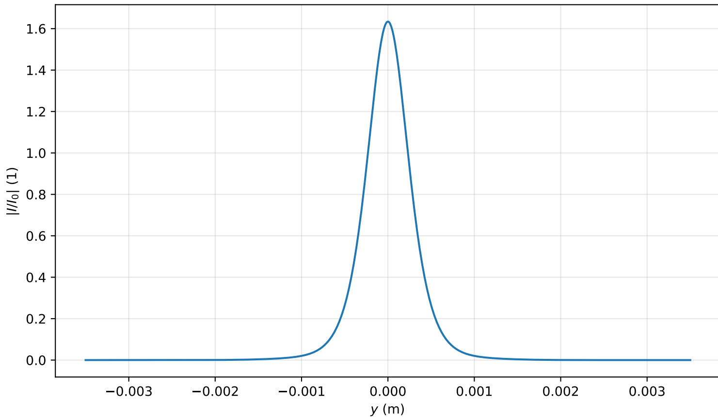
Intensity profile I(x=0, y, z=2.229)/I_0 , P_{in}=0.9P_{cr} , artificial time
